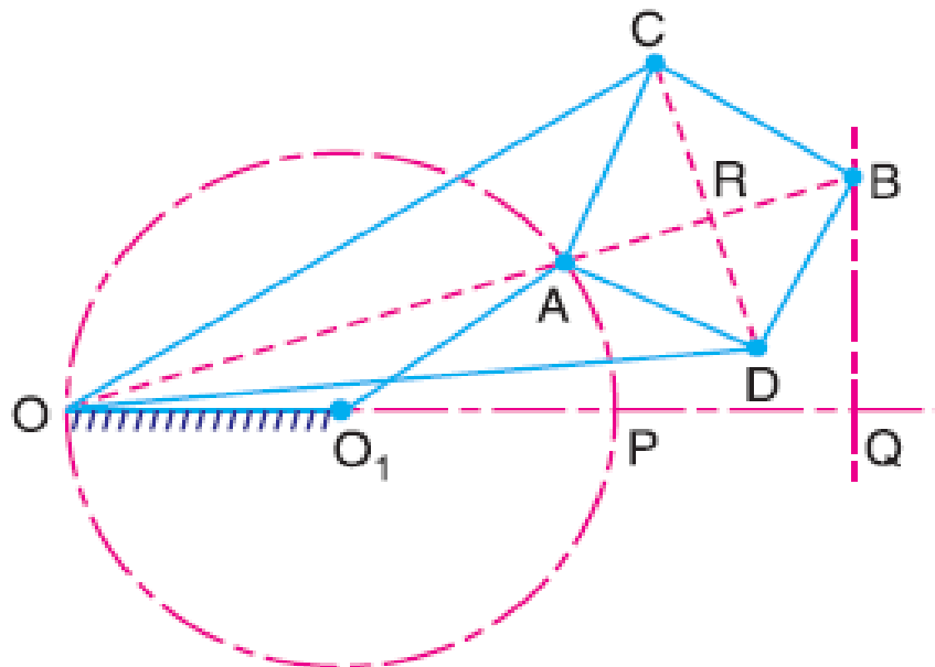
Fig. 4.2 Peaucellier Mechanism
