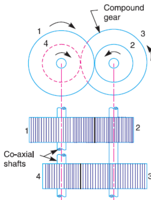
Fig. 5.2.3 Reverted gear train
