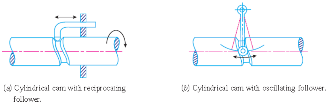
Fig. 4.2 cylindrical cam
