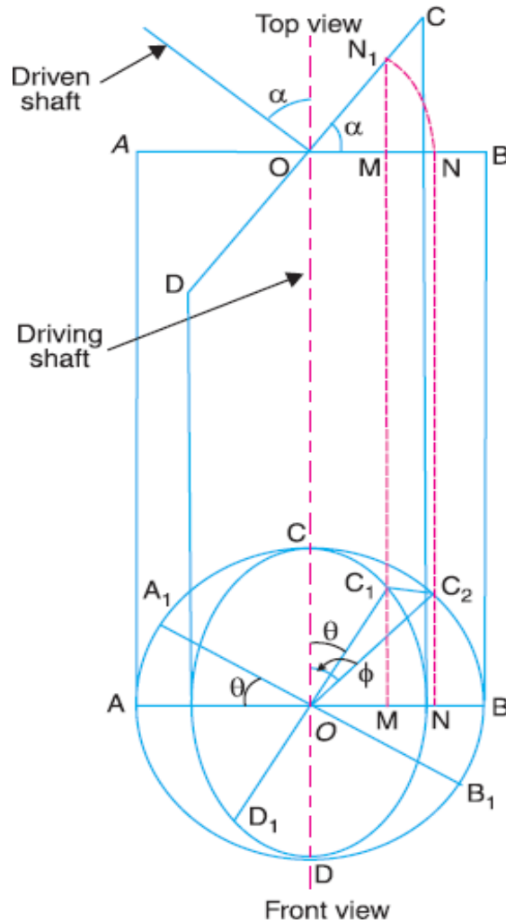
Fig. 4.14 ratio of shaft velocities
