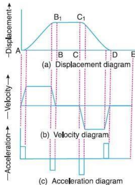
Fig. 4.5 modified displacement, velocity acceleration diagrams
