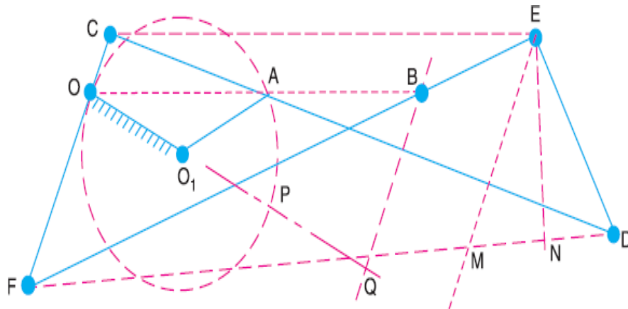
Fig. 4.3 Hart's Mechanism
